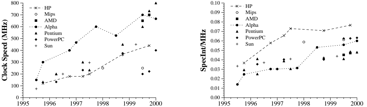
Figure 1: Processor clock rates and normalized processor performance (SpecInt/Clock rate), 1995-2000.
